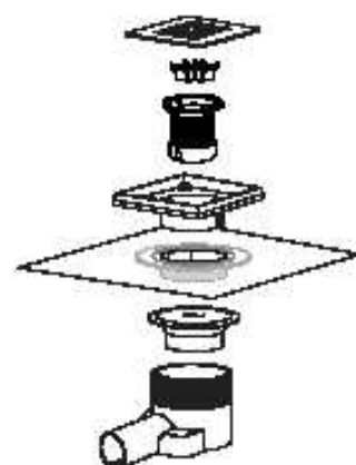
Raindrain Point 56246800 / 56248800
