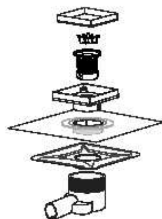
Raindrain Point 56247XX0 / 56249XX0
